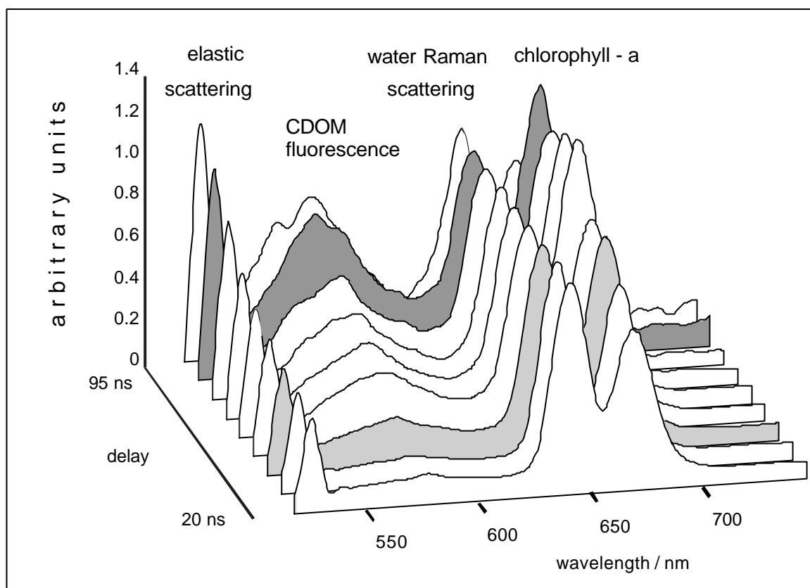
Figure 8: A series of spectra from the tank experiment, taken as a function of the programmed delay.
