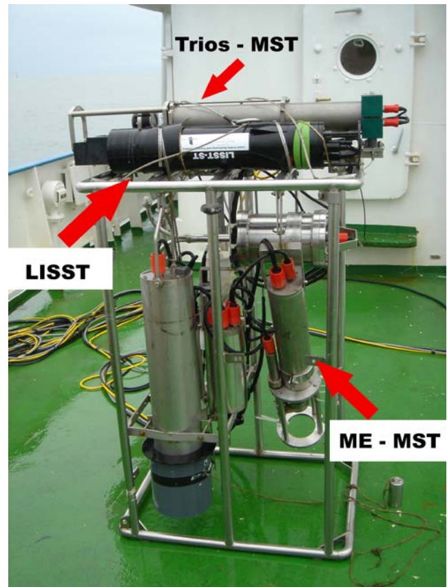
Fig. 4 Photo of instrument setup during research cruise aboard FK Senckenberg in October 2007. CTD, ME-MST, Trios-MST and LISST were mounted to the same frame in order to ensure comparability of measurements
