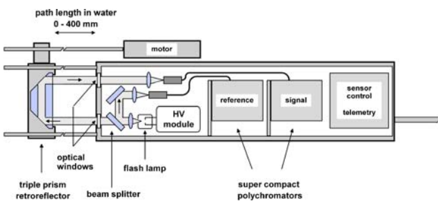
Fig. 3 Schematic representation of the MST
